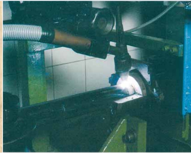
1972 Automatic forming and welding of burner body
